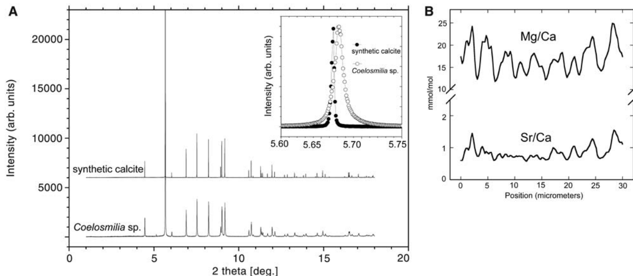
Fig. 3. Crystal structure and chemical composition of the Coelosmilia sp. calcitic skeleton. (A) High-resolution synchrotron radiation powder diffraction patterns of Coelosmilia sp. skeleton (lower trace) and synthetic calcite (upper trace). The most intense (104) Bragg peak is shown in the inset. The Bragg peaks
